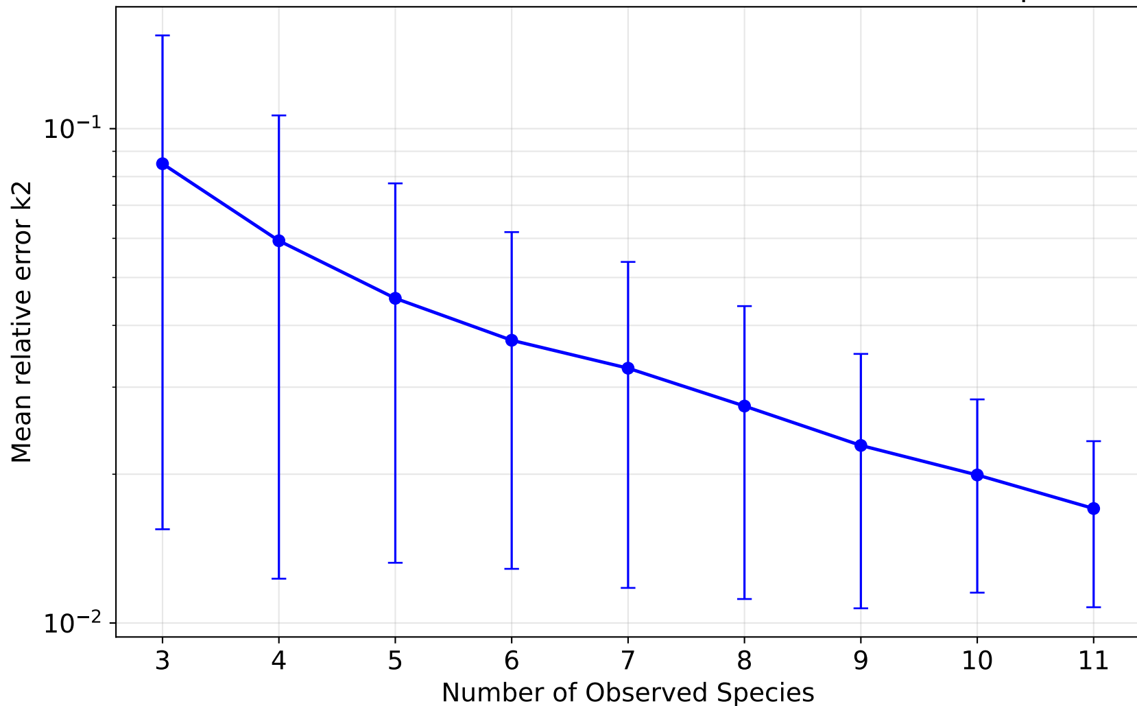
30, 30 — Mean relative error k2 vs number of observed species
